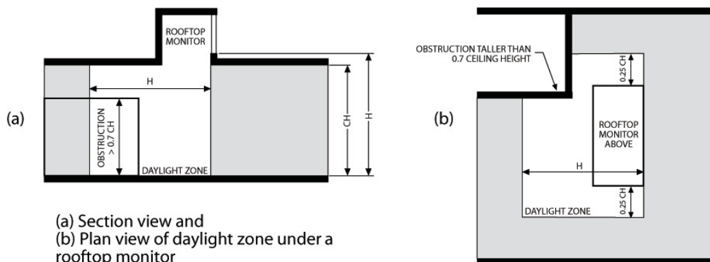
FIGURE C405.2.4.2(2) DAYLIGHT ZONE UNDER A ROOFTOP MONITOR
