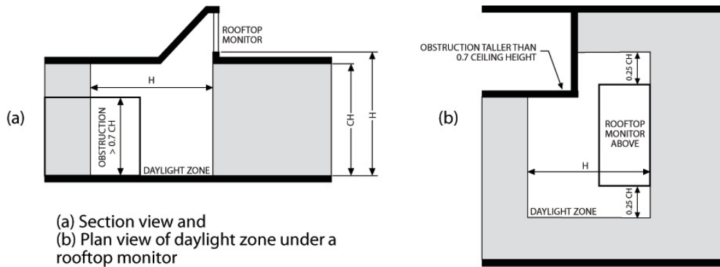
FIGURE C405.2.4.2(3) DAYLIGHT ZONE UNDER A SLOPED ROOFTOP MONITOR
