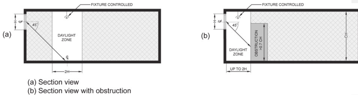
FIGURE C405.2.4.2(4) DAYLIGHT ZONE ADJACENT TO CLERESTORY FENESTRATION IN A WALL
