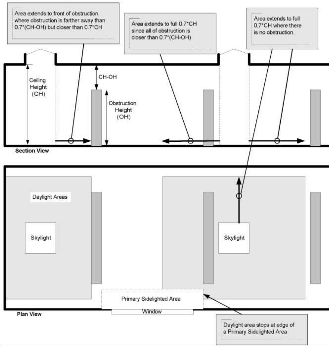
FIGURE C405.2.4.3(1) DAYLIGHT ZONE UNDER A ROOFTOP FENESTRATION ASSEMBLY
