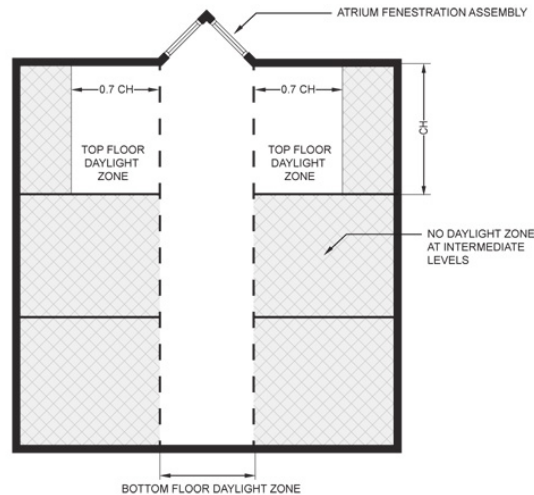
FIGURE C405.2.4.3(2) DAYLIGHT ZONE UNDER ATRIUM FENESTRATION
