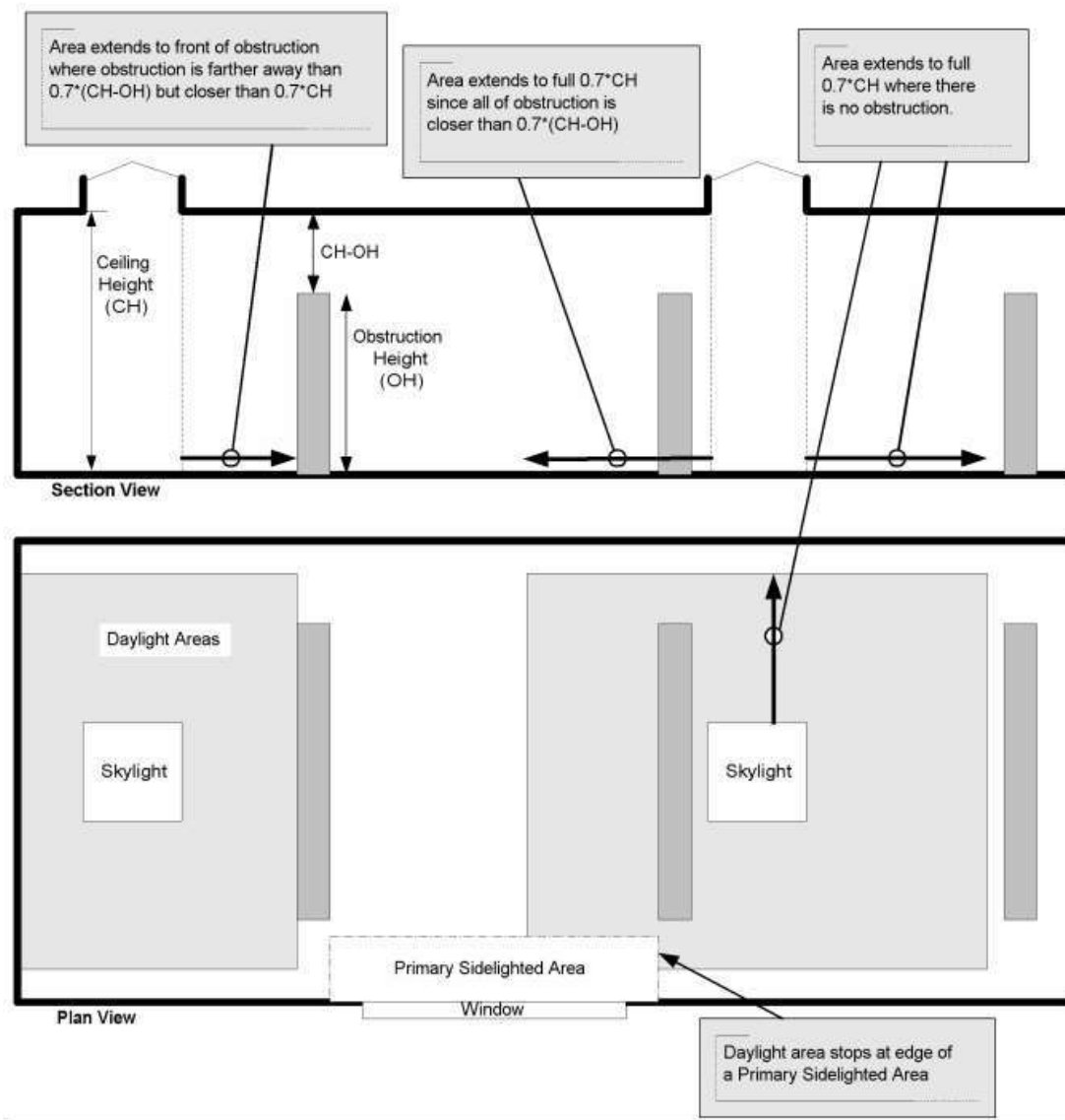
FIGURE C405.2.4.3(1) DAYLIGHT ZONE UNDER A ROOFTOP FENESTRATION ASSEMBLY
