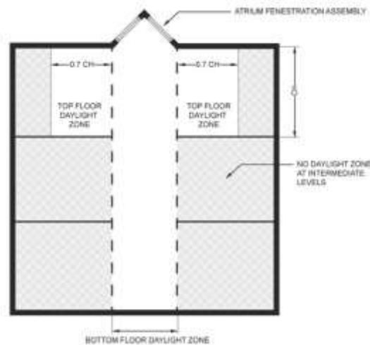
FIGURE C405.2.4.3(2) DAYLIGHT ZONE UNDER ATRIUM FENESTRATION
