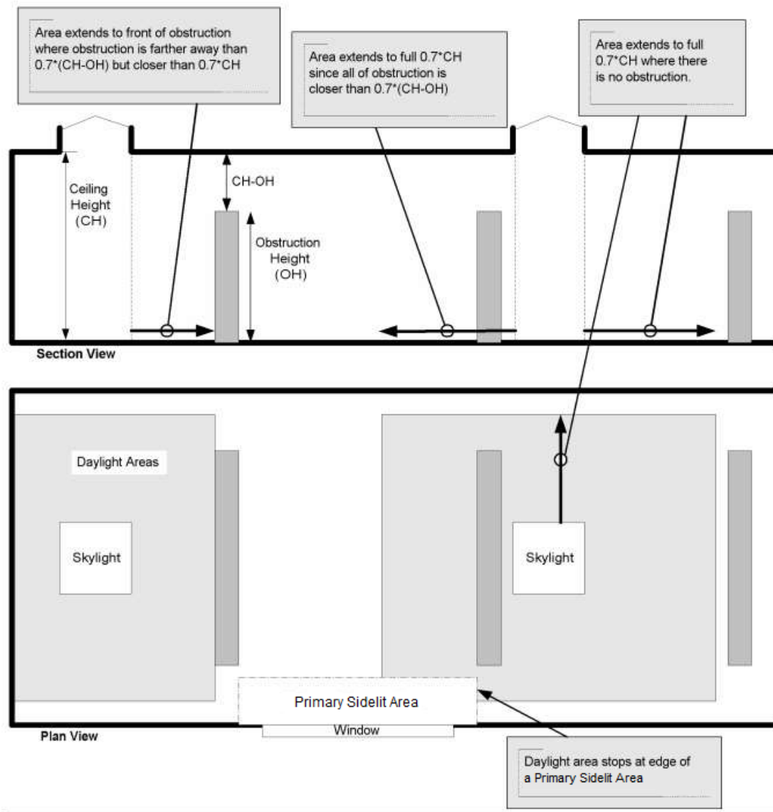
FIGURE C405.2.4.3(1) DAYLIGHT TOPLIT ZONE UNDER A ROOFTOP FENESTRATION ASSEMBLY
