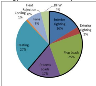
Energy end-use summary - school building
