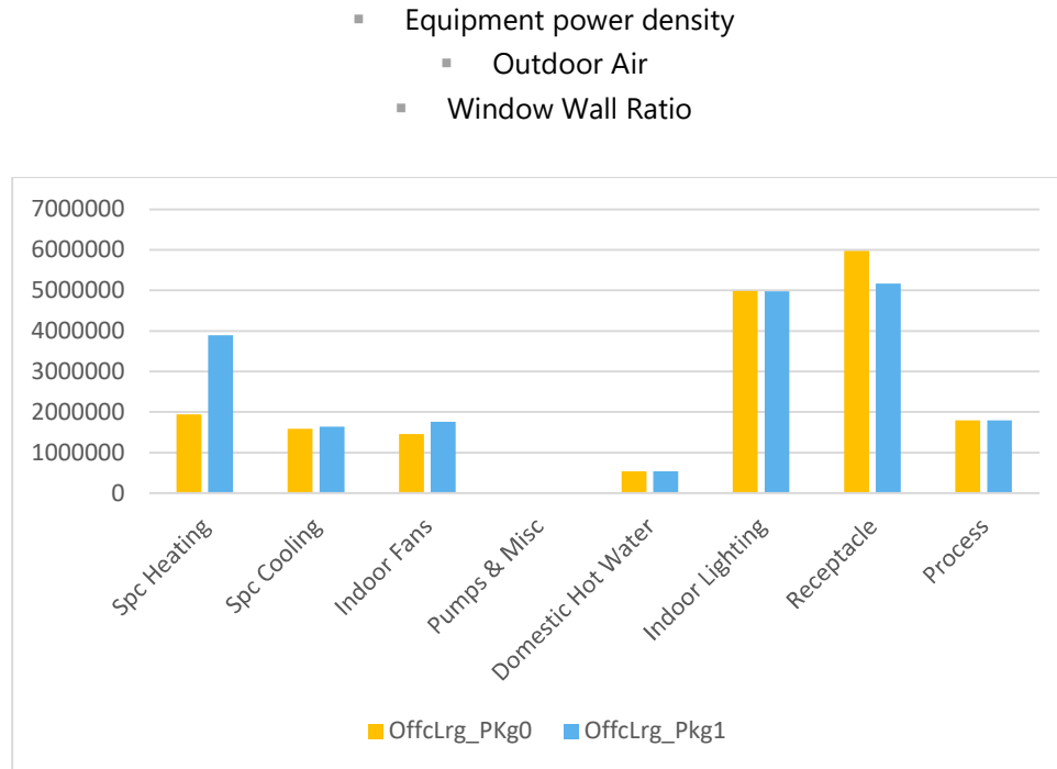
Figure 12. Updated total energy [kBtu/yr] for Large Office in 2006 baseline by end-use
