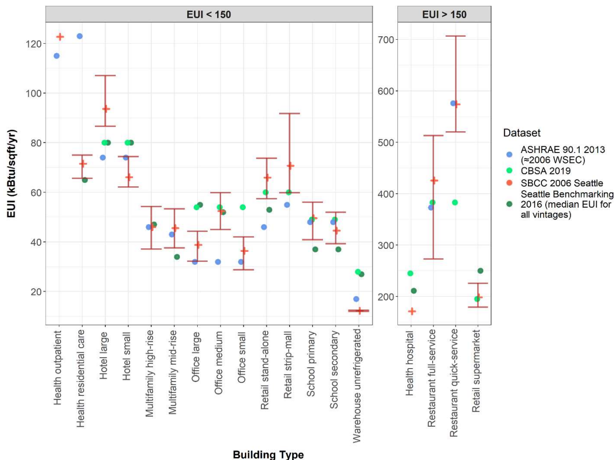
Figure 14. 2006 baseline model average EUI variation due to unregulated loads (4C Climate) with Comparison Datasets
