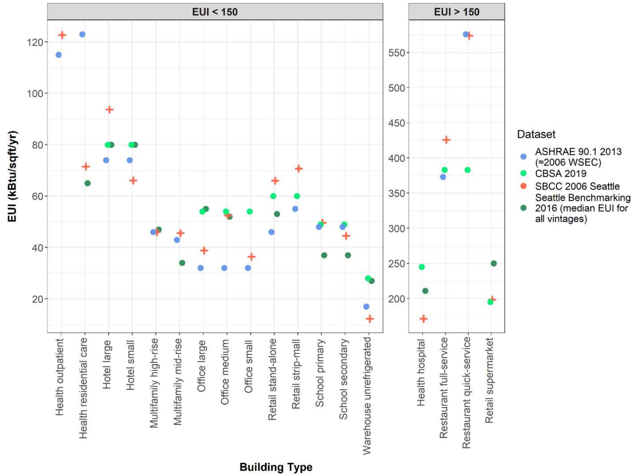
Figure 6. Phase One 2006 Commercial Building Modeling Results (4C Climate) with Comparison Datasets
