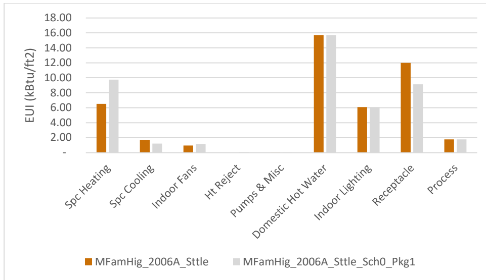
Figure 7. Updated High-Rise Multifamily results for 2006 baseline by end-use
