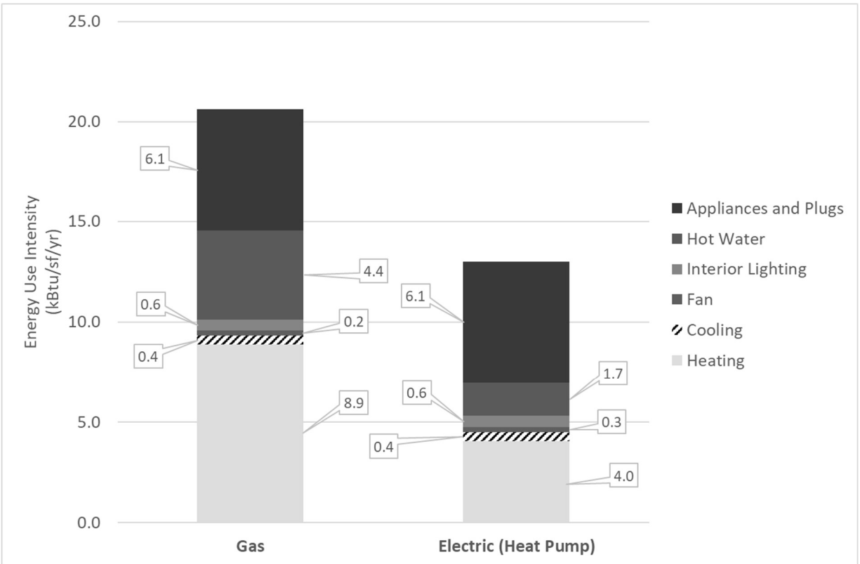
Figure 5. Average Modeled EUI of a Single-Family Dwelling (by EUI) in 2018 – Gas vs Electric Heating Source
