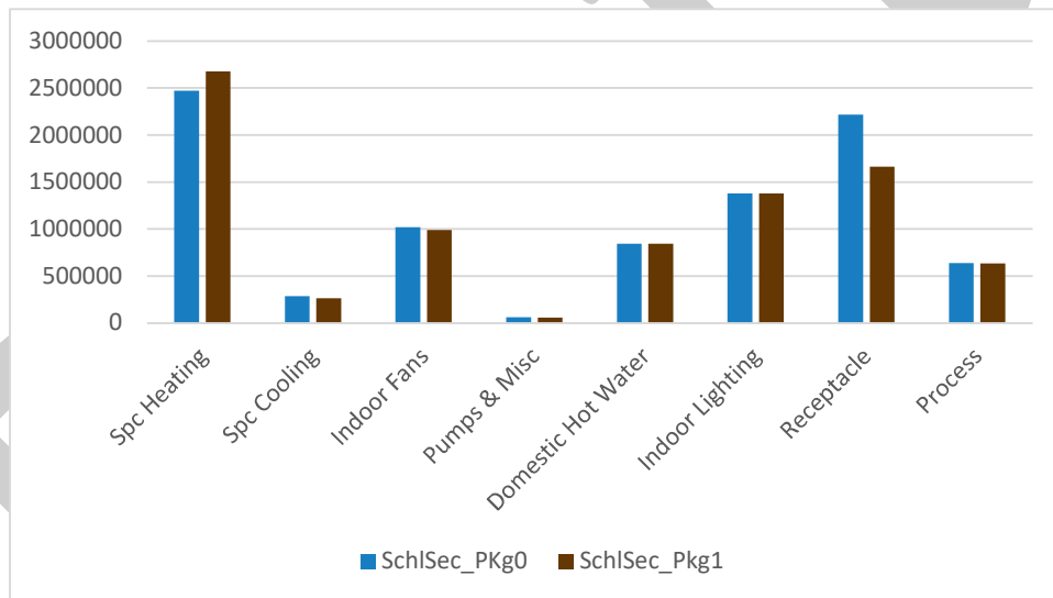
Figure 11. Updated total energy [kBtu/yr] for Secondary School in 2006 baseline by end-use
