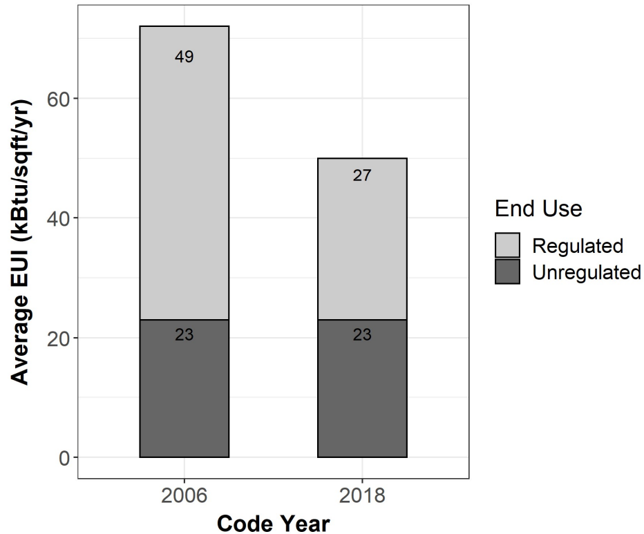
Figure 16. State Comparison Including Regulated and Unregulated End Uses
