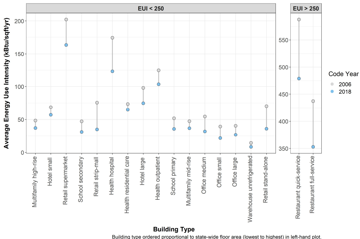
Figure 15. Commercial Modeled EUI Comparison by Building Type by Code Year (needs update)
