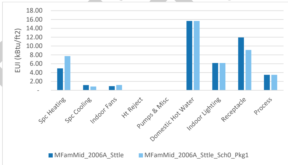
Figure 8. Updated Mid-Rise Multifamily results for 2006 baseline by end-use
