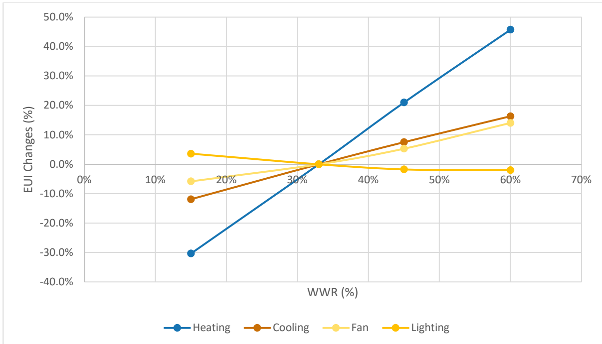
Figure 13. Impact of change in WWR on end-use energy for 2006 Medium Office prototype
