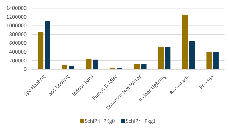
Figure 10. Updated total energy [kBtu/yr] for Primary School in 2006 baseline by end-use
