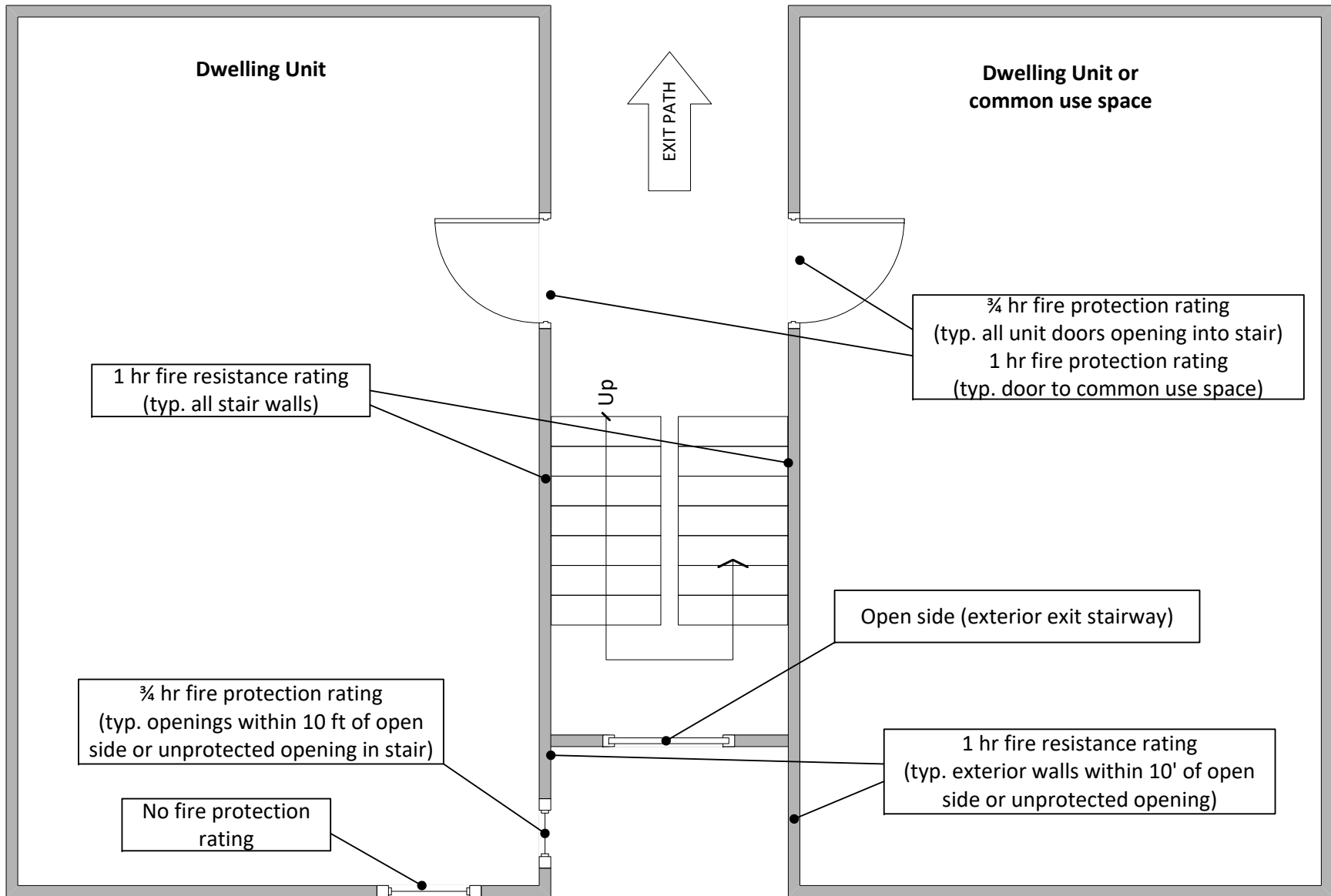
Fig. XX104.1(3) - 3-story Building, Exterior Stair Ground Level
