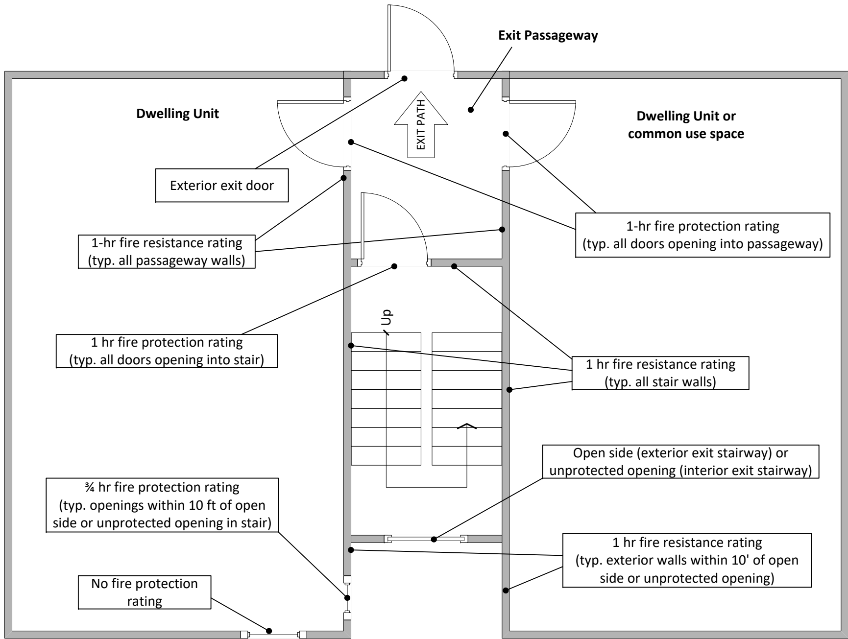
Fig. XX104.1(4) - 3-story Building - Interior Stair Ground Level
