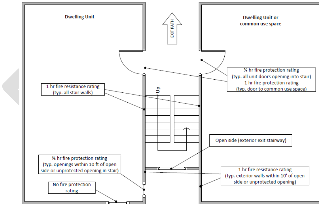
Fig. XX104.1(3) - 3-story Building, Exterior Stair Ground Level
